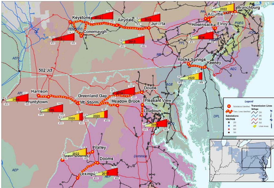
Map Highlighting Critical Overloads over the 2012-2022 Planning Horizon and the Year the Overload Occurs
